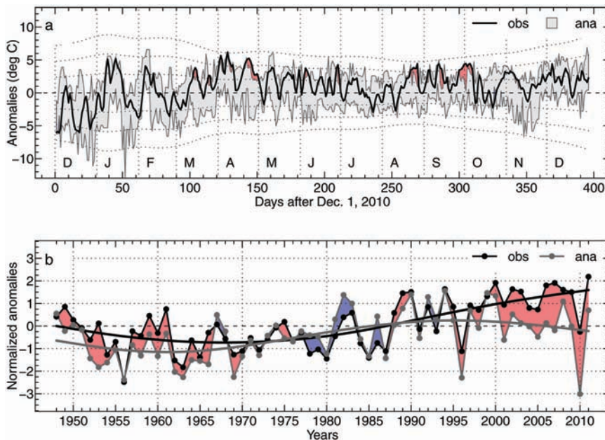
FIG. 11. (a) Daily anomalies ( ^{\circ} C) of observed (black line) and analog (gray spread encompassing the 10 values) temperatures from December 2010 to December 2011. Dashed lines indicate climatological \sigma levels (higher variability in winter than in summer), and red (blue) indicates days with observed temperatures above (below) the 10 analog values. (b) Yearly observed (black) and analog (gray) temperatures averaged over western Europe, represented as normalized anomalies relative to the period 1971–2000. Smoothing by splines with 4 degrees of freedom is added, and red (blue) indicates years with observed temperatures above (below) analog ones. The recent tendency for observed temperatures to be warmer than analog temperatures is particularly prominent in both 2010 (cold record in analogues while close to normal in observations) and 2011 (warm record in observations while <1\sigma in analogues).
